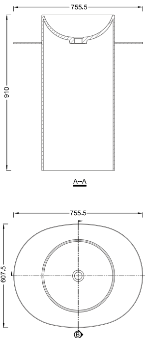
RLH-B4002 SIZE:755.5mm×607.5mm×910mm
