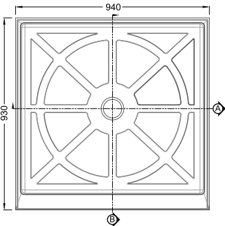
RLF133 SIZE:940mm×930mm×127mm
