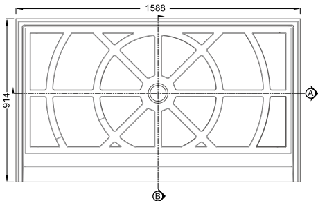
RLF135 SIZE:1588mmx914mmx127mm
