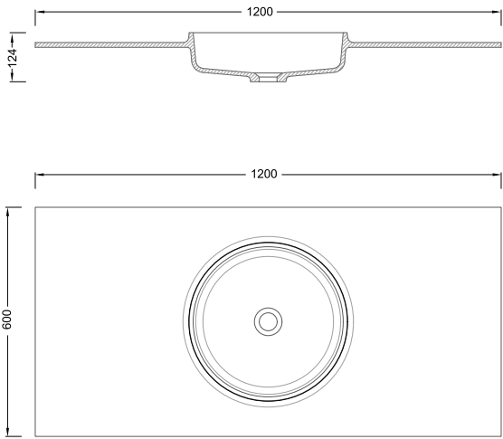
GDRLX001 SIZE:1200mmx600mmx124mm
