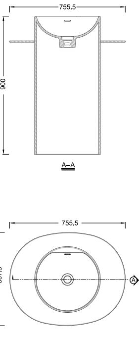
RLH-B4001 SIZE:755.5mmx607.5mmx900mm
