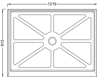
RLF134 SIZE:1219mmx914mmx133mm
