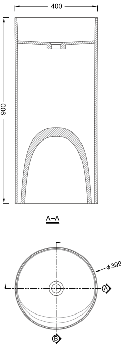
RLZ141 SIZE:400mm×399mm×900mm
